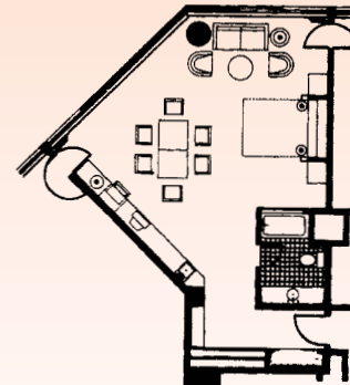
D. Deluxe Bedroom 690 sq. ft.
